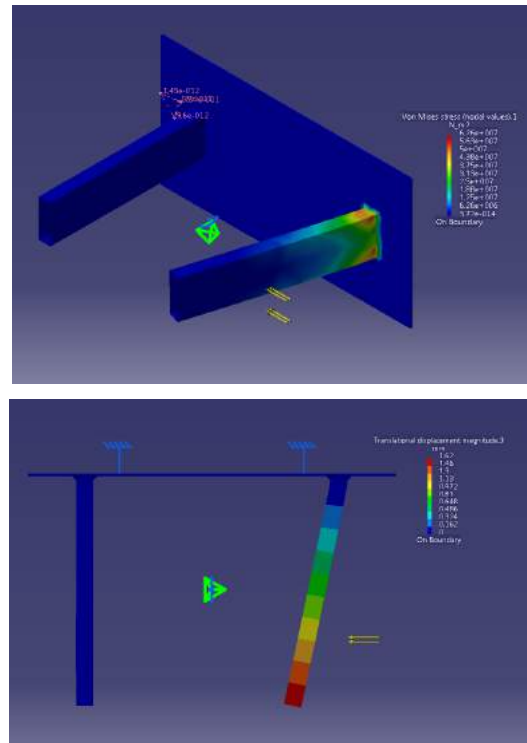
Figure 44. Representation of sidemembers as cantilever beam.
