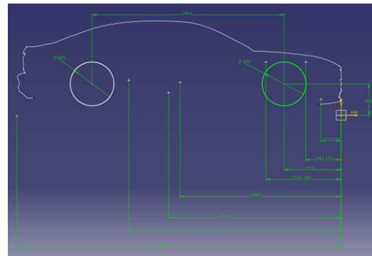
Figure 6. General dimensions of the car
