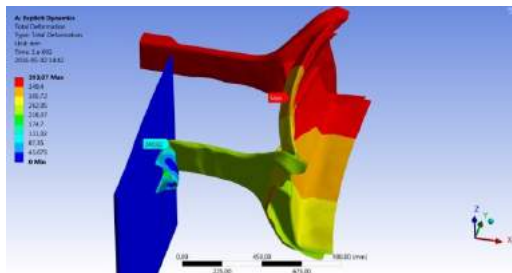
Figure 30. Total deformation of the sidemembers, plate elements model
