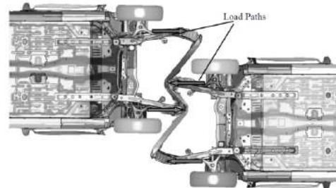
Figure 18. Fork effect on two collapsing vehicles car-to-car misalignment. Reza and Simkus, 2011, Chalmers
