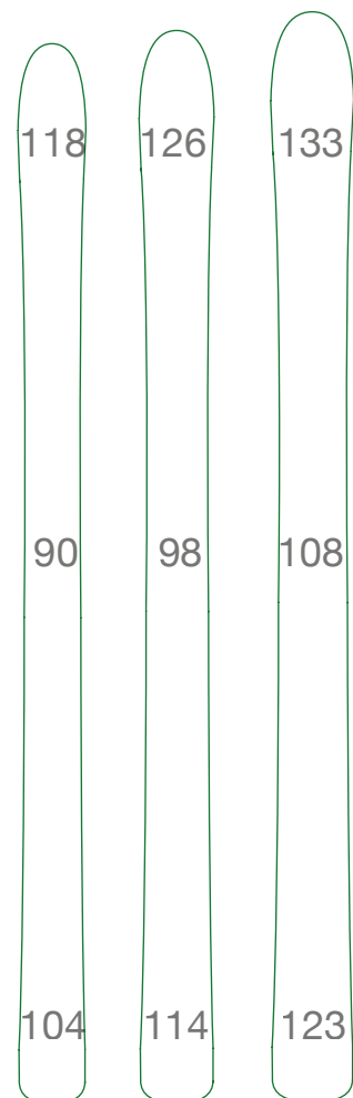
Figure 52. Constructional drawings of rocker length, camber and boot centre (top left), flex (middle left), measurements (down left), constructive drawing of shape (right)
