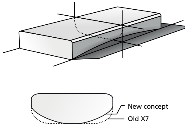
Figure 4.6 Concave shape like Trimble Nomad, and the most comfortable section shape
